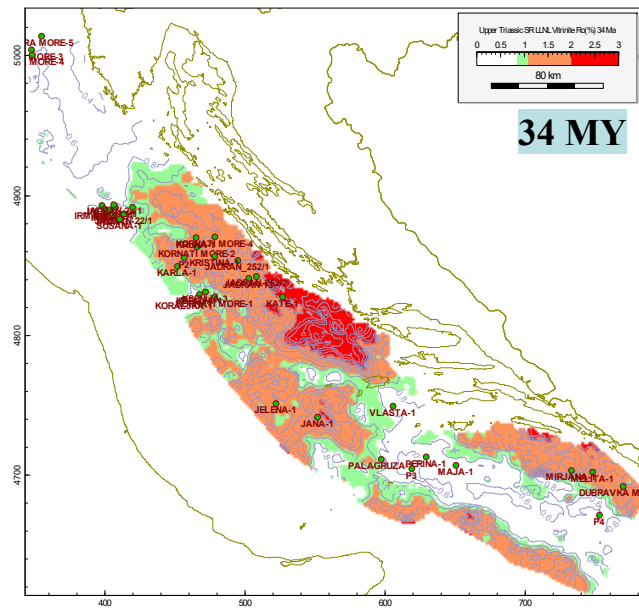
Maturity history for Upper Triassic source rock. (Maturity Window)
