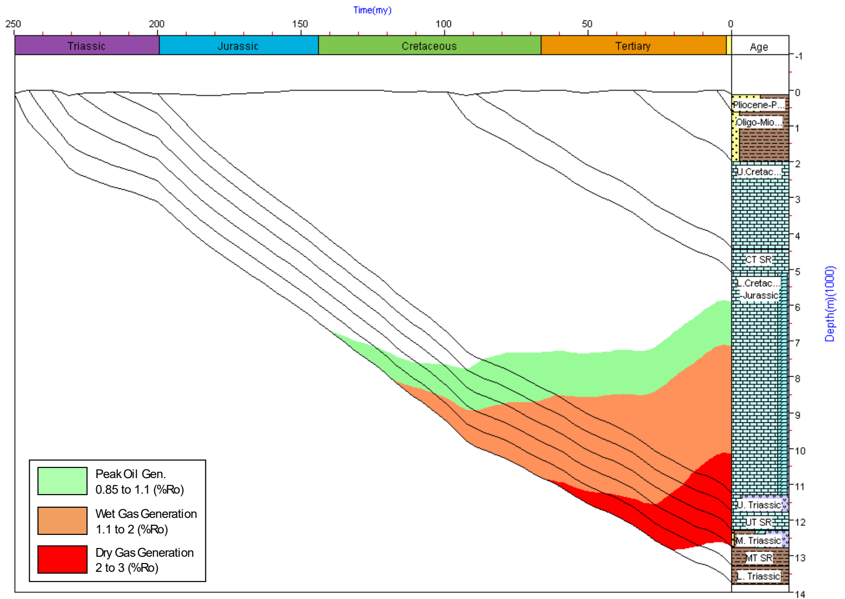
Burial history curve for Kate-1 well.
